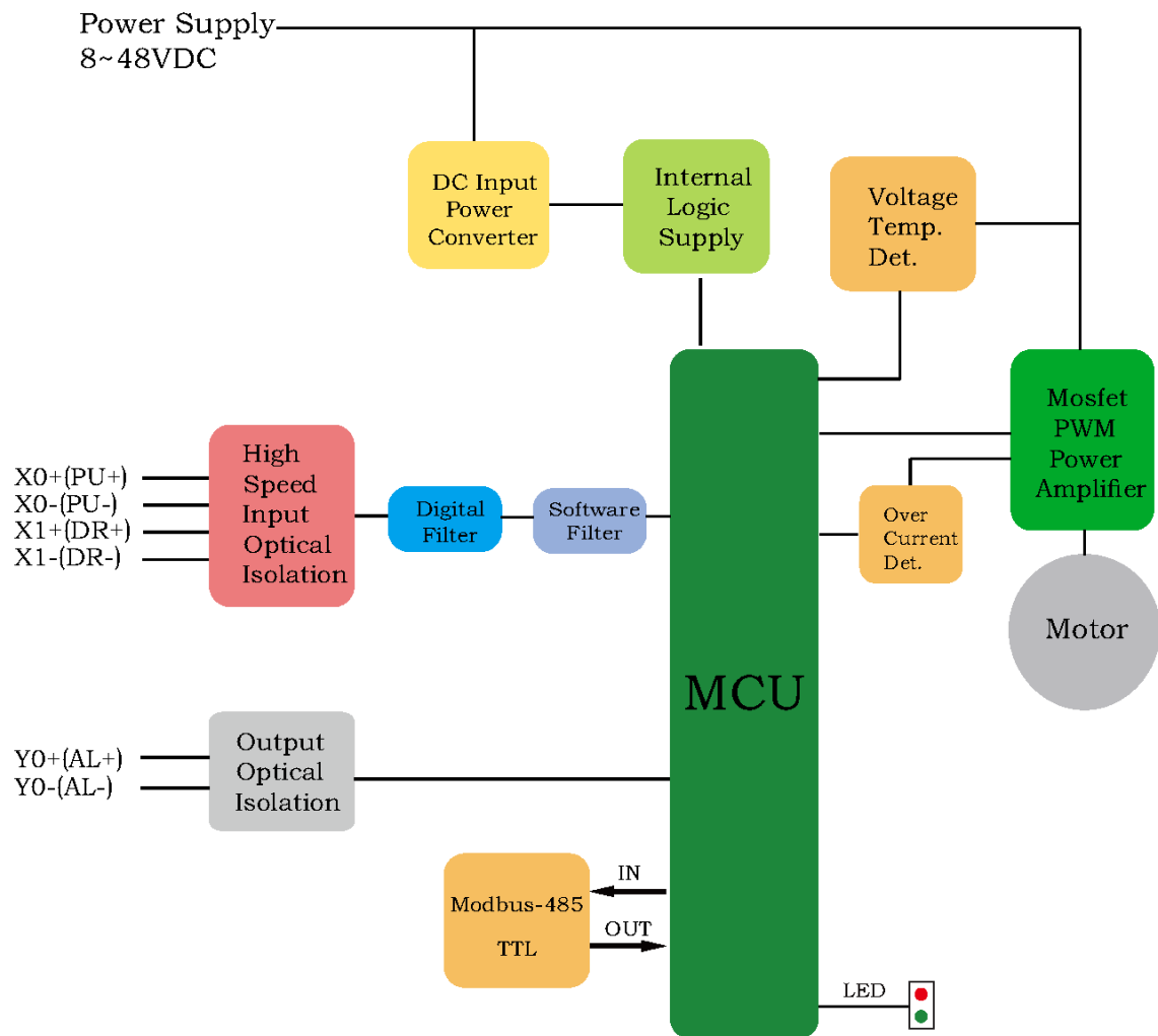
Block Diagram
